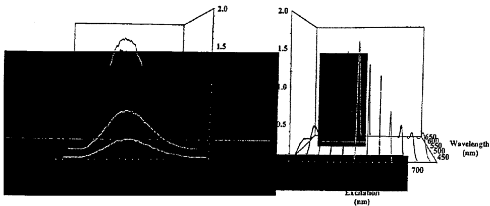
Figure 4 Two-photon upconverted fluorescence emission spectra of 1 at several fs pulsed pump wavelengths ( 2.5 \times 10^{-4}\text{M} , ACN).
