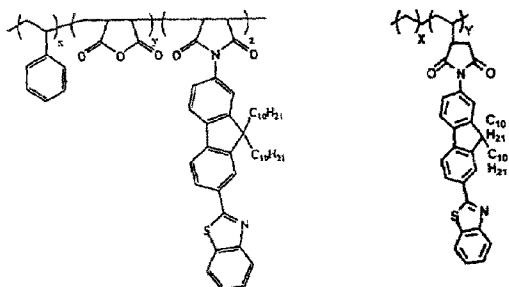
Figure 14. Structure of photosensitive polymers.
