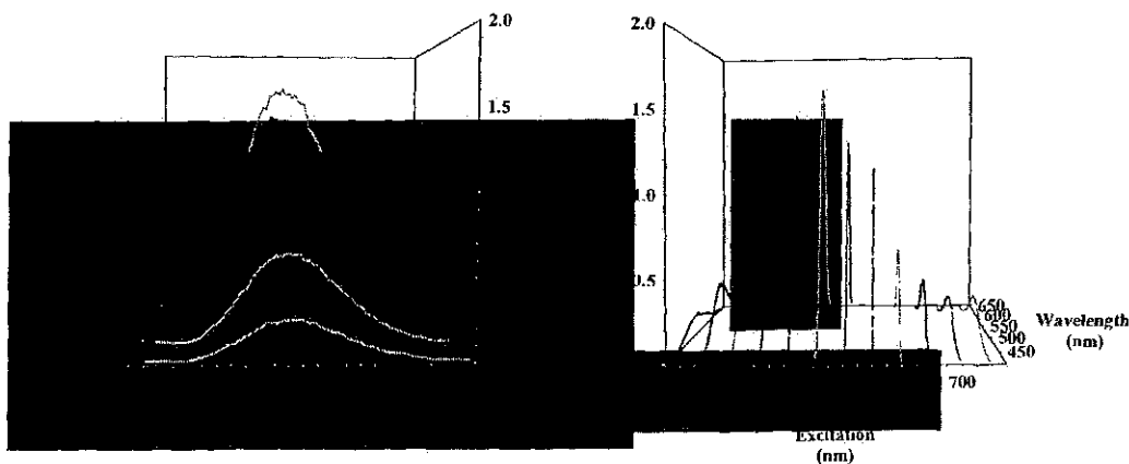
Figure 4 Two-photon upconverted fluorescence emission spectra of I at several fs pulsed pump wavelengths ( 2.5 \times 10^{-4} \text{ M} , ACN).
