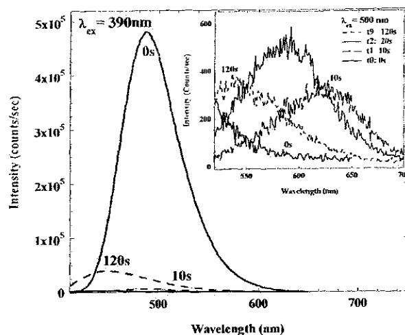
Figure 3 is a graphical representation of the time-dependent fluorescence emission spectra for the photolysis of fluorene I and photoacid generator in \text{CH}_2\text{Cl}_2 at photolysis times from 0 to 120 sec (excitation at 390 nm) with an inset that shows fluorescence at longer wavelength with excitation at 500 nm.
