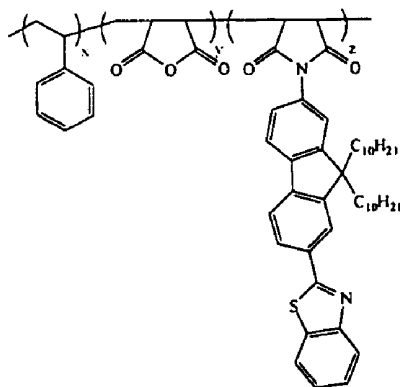
Structure of photosensitive polymers.
