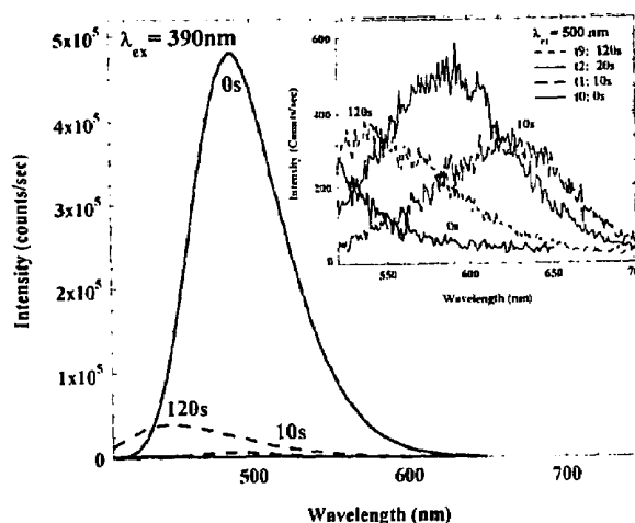
Figure 3 is a graphical representation of the time-dependent fluorescence emission spectra for the photolysis of fluorene 1 and photoacid generator in CH 2 Cl 2 at photolysis times from 0 to 120 sec (excitation at 390 nm) with an inset that shows fluorescence at longer wavelength with excitation at 500 nm.
